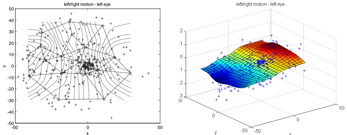
Figures 5. Left: the input space (in image space coordinates). The '+' signs represents training examples, and the circles are the position of unit's centers; contour lines are also shown. Right: one of the components of the output vector for the same training set. The plot has been obtained after about 90000 steps performed using a 300 samples wide training set.
